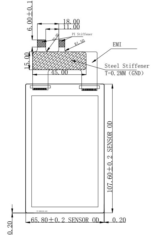
Back View
