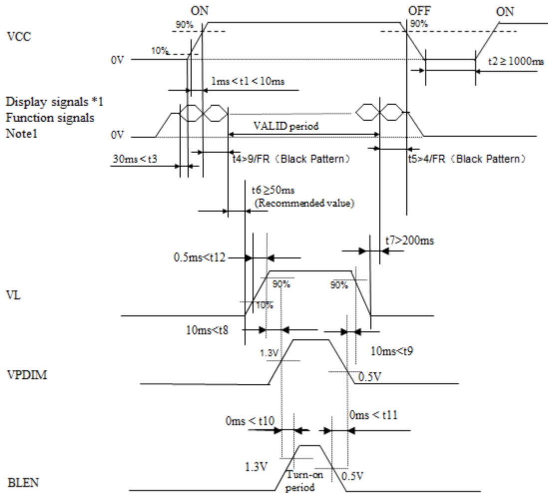
Figure 5.3.1 Power On/off sequence
