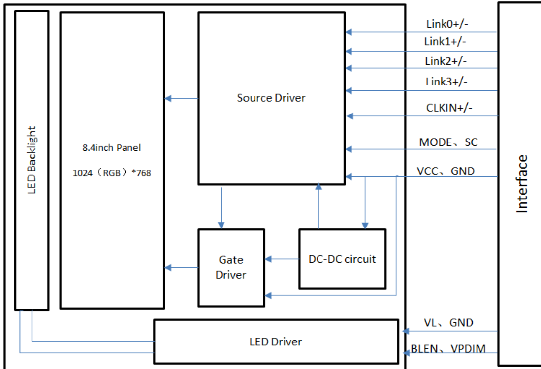
Figure 5.4.1 LCD Module Block Diagram
