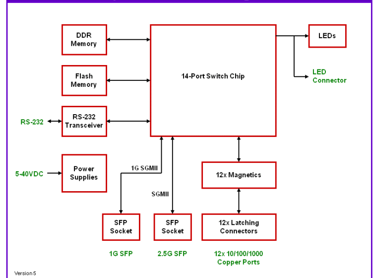
Epsilon-12G2 Block Diagram
